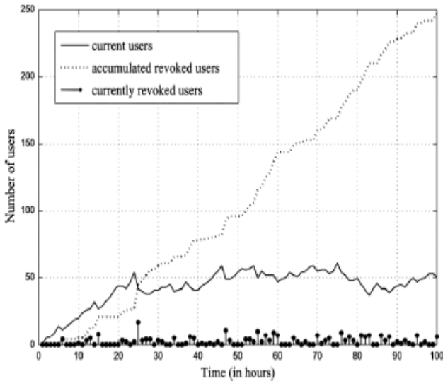
Fig. 2. Number of users in an attribute group.
