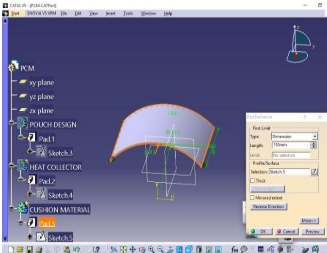
Fig5. 3-D View of Vinyl Cushion.
