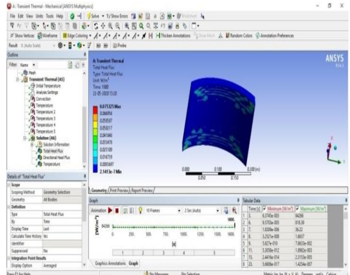
Fig14. Total Heat Flux.
