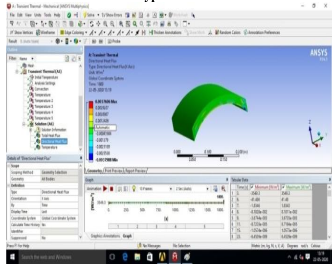
Fig13. Directional Heat Flux.
