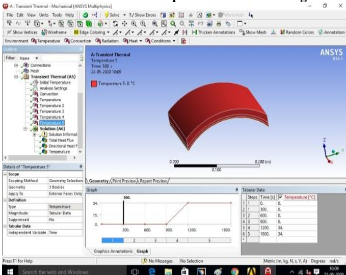
Fig10. Temperature applied on PCM at 34°C.
