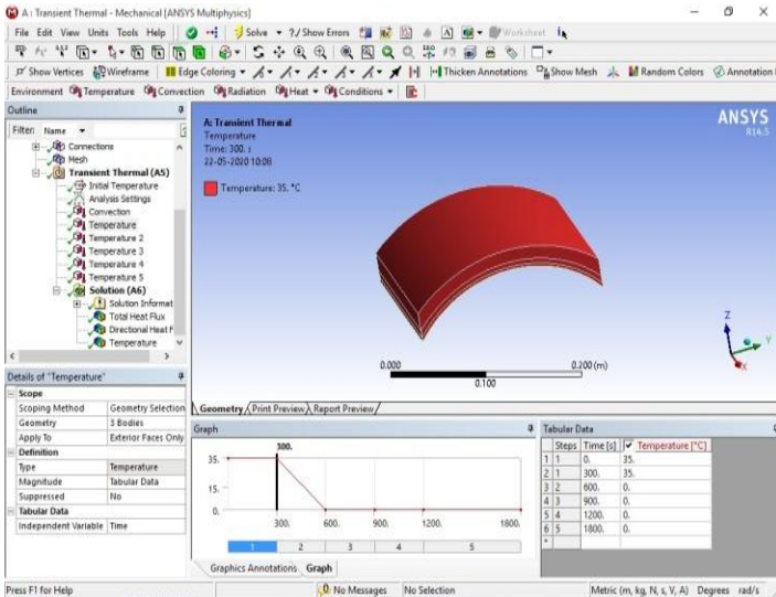
Fig11. Temperature applied on PCM at 35°C.
