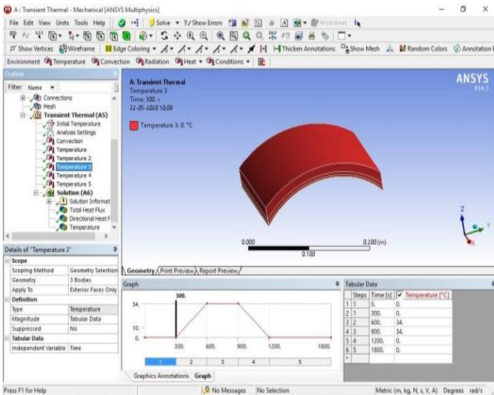
Fig12. Temperature applied on PCM at 36°C.
