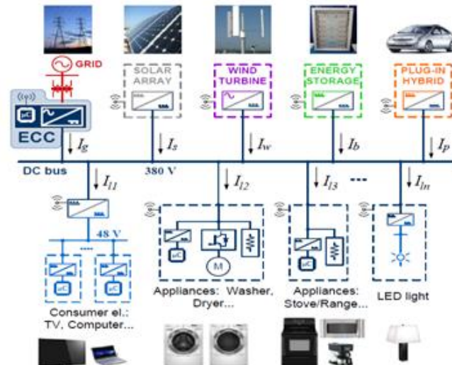
Fig.1. Configuration of the proposed dc microgrid system with EMS.
