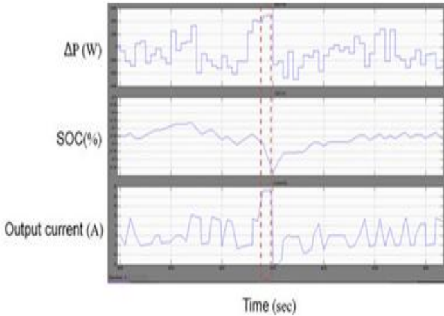
Fig.13. Simulation results when the bidirectional inverter rating is over the power rating.
