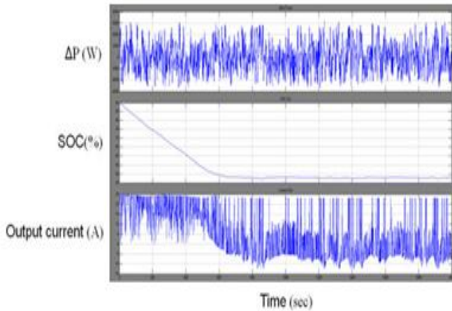
Fig.12. Simulation result with initial battery SOC at 90%.
