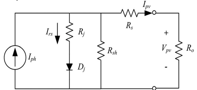
Fig. 2. Solar panel equivalent circuit.
