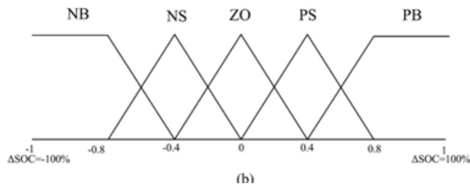
Fig.8. Input membership functions of variables: (a) \Delta P and (b) \Delta SOC .
