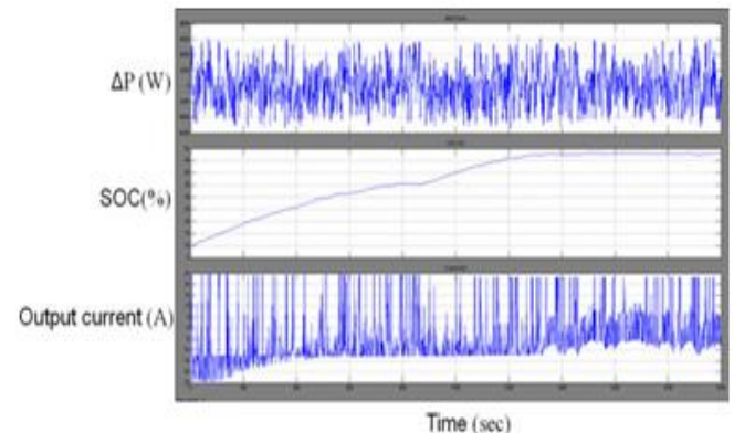
Fig.11. Simulation results with initial battery SOC at 10%.
