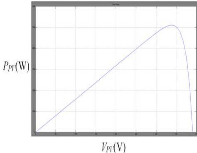
Fig.3. Simulated output power P_{PV} versus output voltage V_{PV} of the solar cell with constant illumination intensity 1 kW/m 2 .
