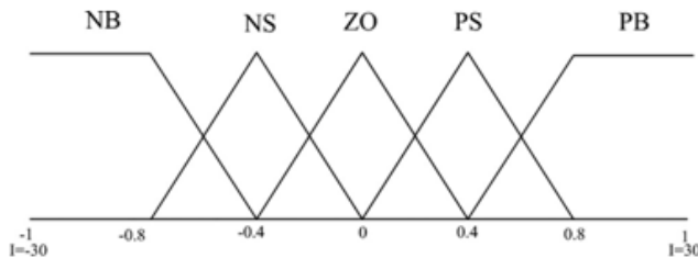
Fig. 9. Output membership function of variable \Delta I .
