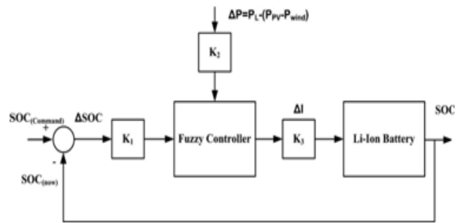
Fig.7. Block diagram of fuzzy control to maintain the desired SOC of the battery.
